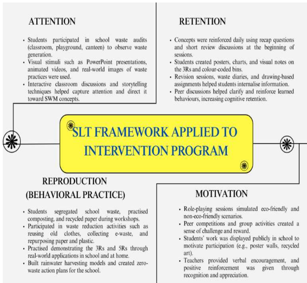
Figure 1 – SLT Framework
