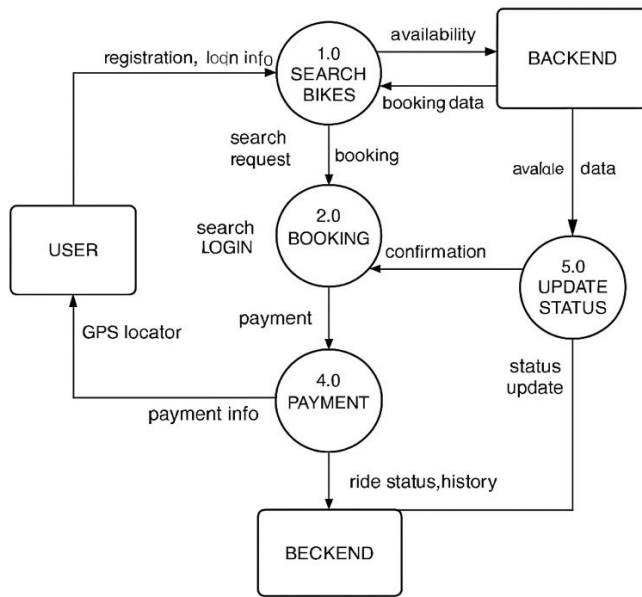
DATA FLOW DIAGRAM LEVEL 1)
