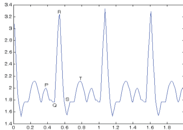
Figure 3. Sinus Tachycardia.
