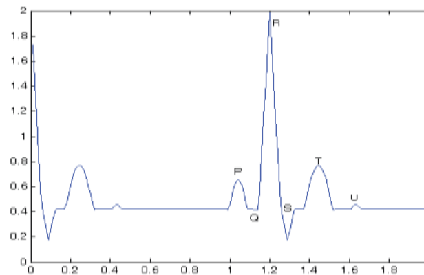
Figure 4. Sinus Bradycardia.
