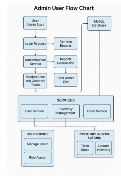
Fig 1. Data flow Diagram(lvl1)
