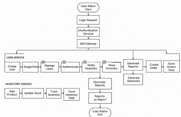
Fig. 2 Data flow diagram (level 2)
