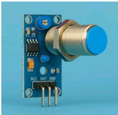
Fig 3: Metal sensor
