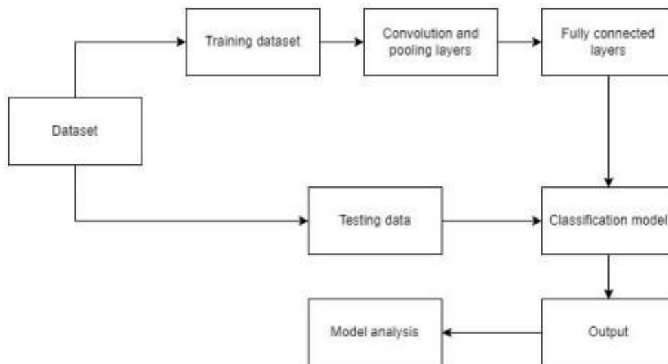
Figure 1: System architecture
