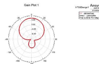
Figure.8. Radiation pattern
