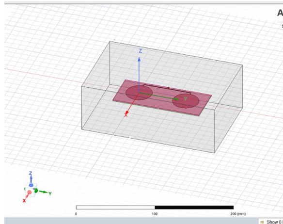
Figure .4. Two element Planer array HFSS model
