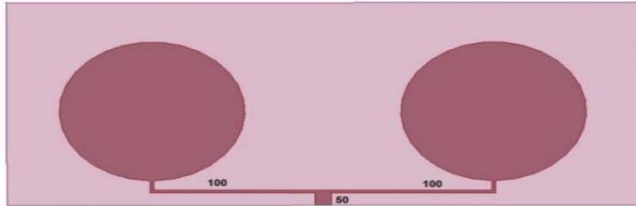
Figure.1. Two elements corporate feed microstrip antenna array
