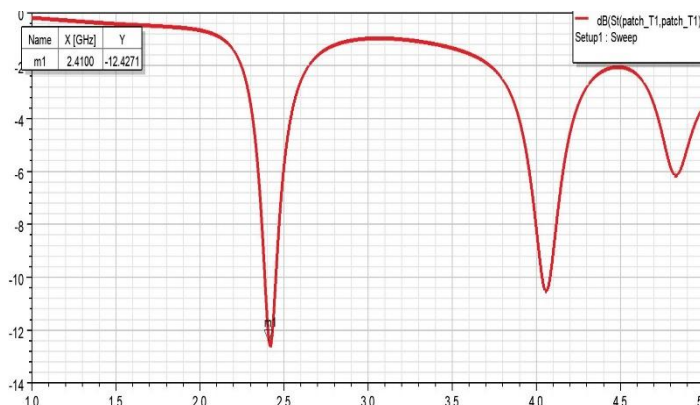
Figure.6. Return loss
