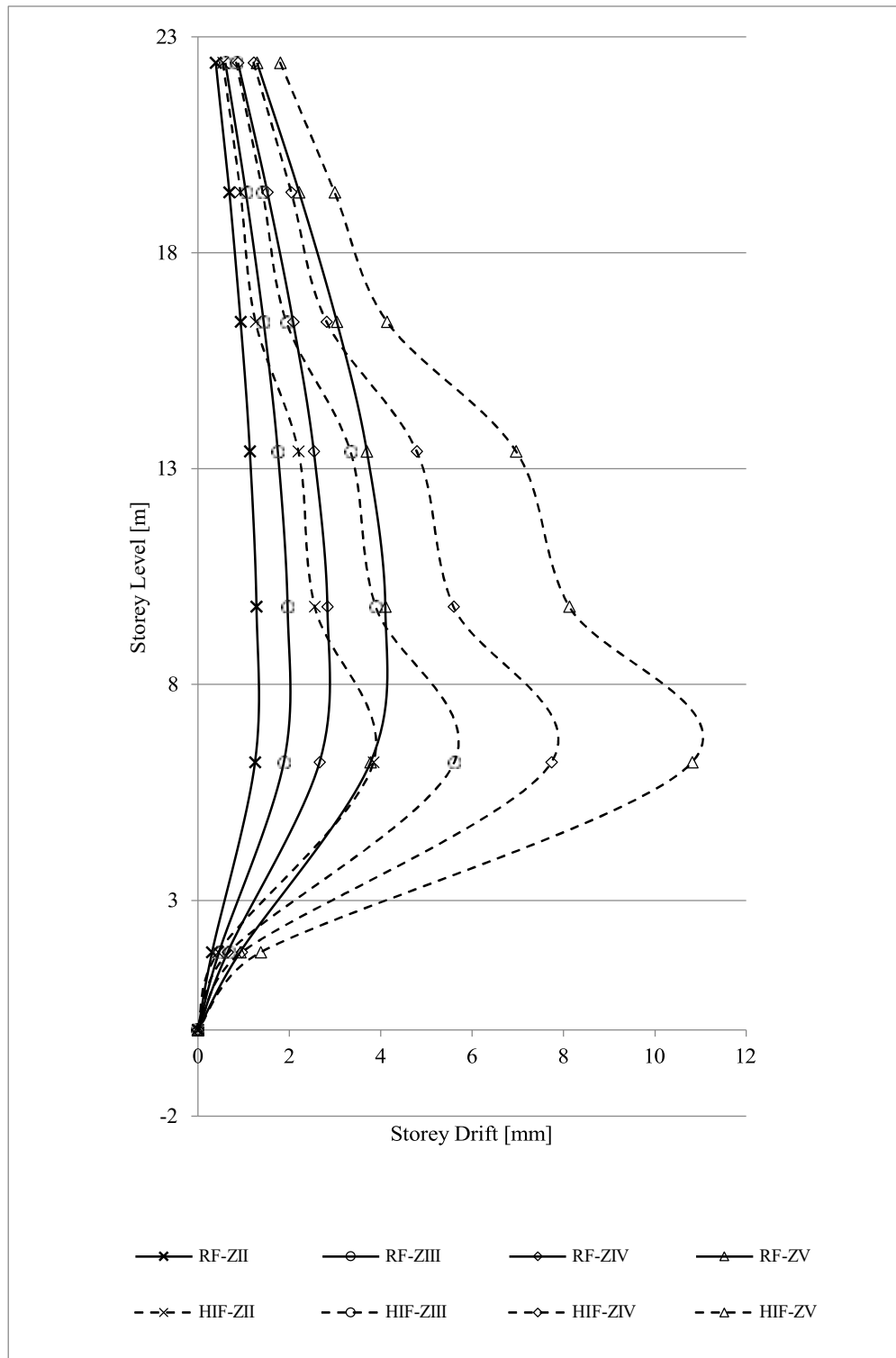
Fig. 4.8 Storey Drift Response of Regular (RF) and Hybrid Irregular (HIF) Frames under Seismic Loads
