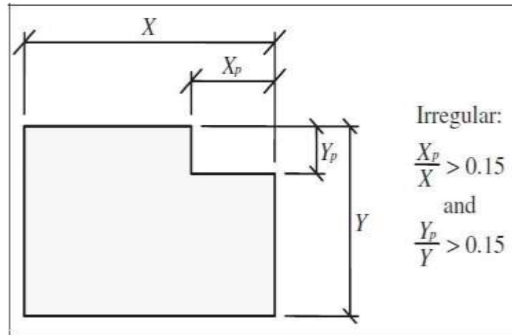
Fig. 1.2 Re-entrant irregularity
