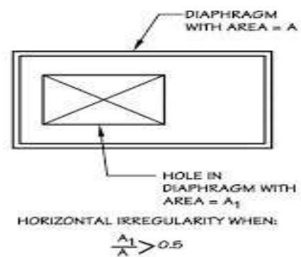
Fig. 1.3 Diaphragm Discontinuity
