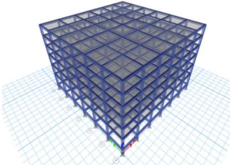
Fig. 3.3 (c) Isometric View of HIF
