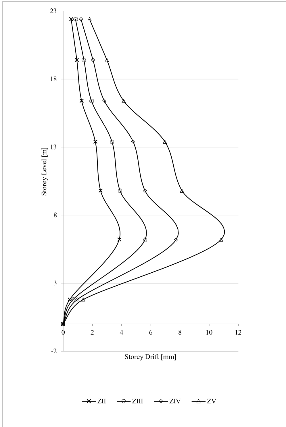
Fig. 4.5 Seismic Response (Storey Drift) of Hybrid Irregular Frame – HIF at all Seismic Zones in India
