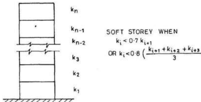
Fig. 1.6 Stiffness Irregularity
