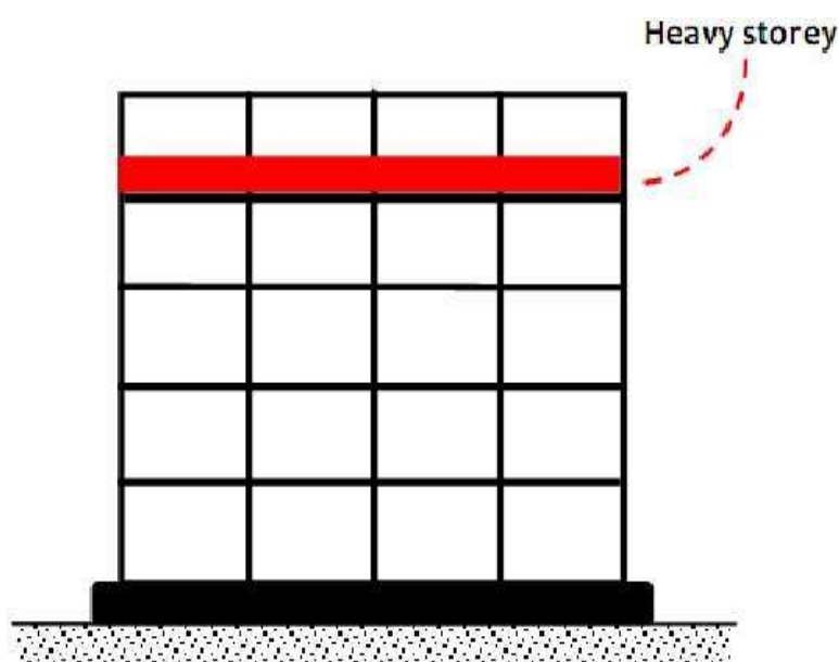
Fig. 1.7 Mass Irregularity
