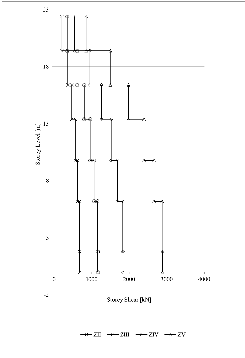
Fig. 4.6 Seismic Response (Storey Shear) of Hybrid Irregular Frame – HIF at all Seismic Zones in India
