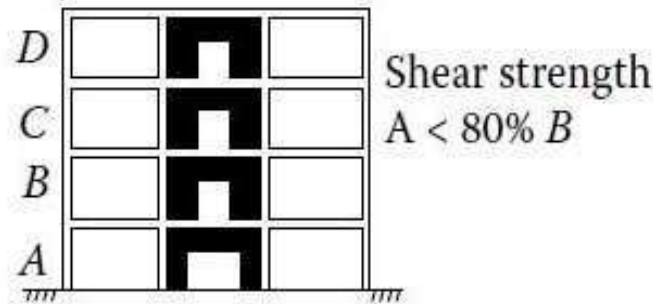
Fig.1.10 Discontinuity in Lateral Strength weak storey Irregularity
