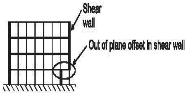
Fig. 1.4 Out of plane Offset Irregularity
