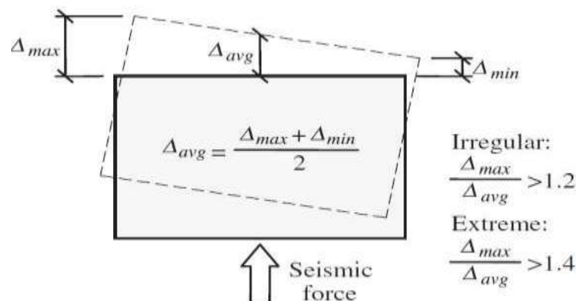
Fig. 1.1 Torsional irregularity
