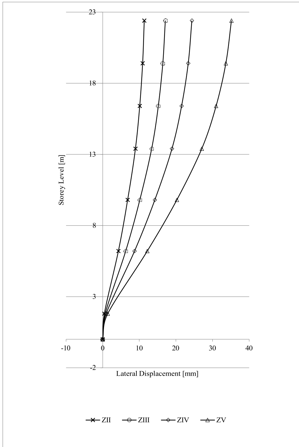
Fig. 4.4 Seismic Response (Lateral Displacement) of Hybrid Irregular Frame – HIF at all Seismic Zones in India
