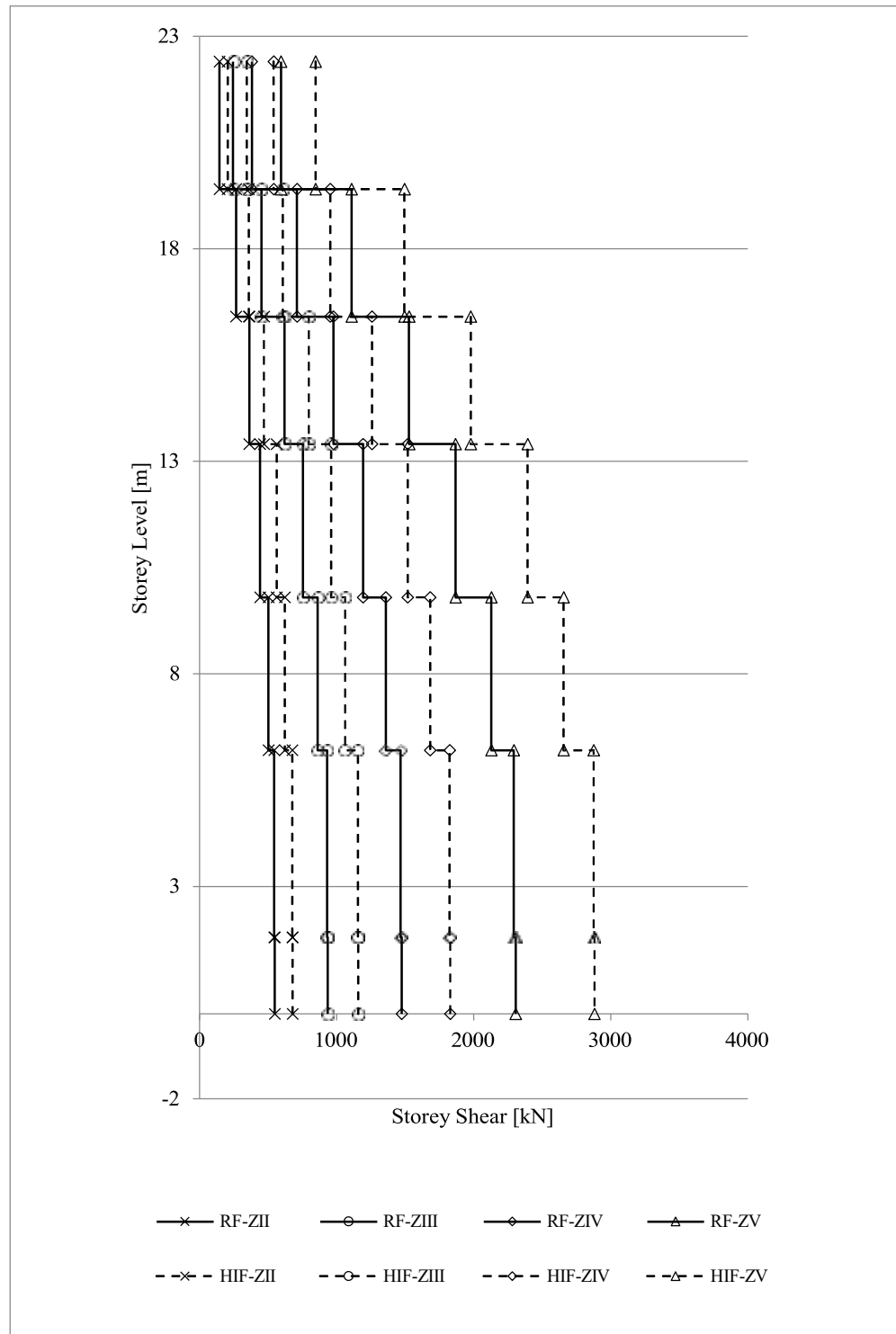
Fig. 4.9 Storey Shear Response of Regular (RF) and Hybrid Irregular (HIF) Frames under Seismic Loads
