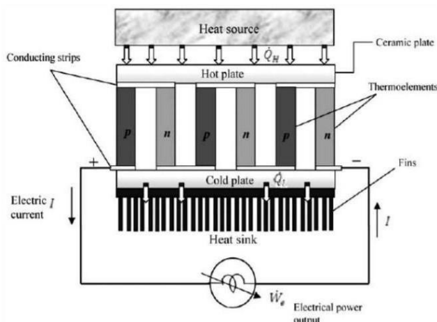
Figure 1.2 Typical Single-Stage Thermoelectric Power Generator
