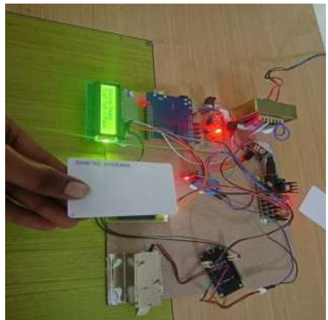
Fig.5.Door Unlocks
