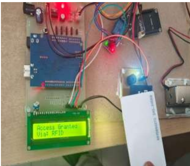
Fig. 9. Authorized Tag
