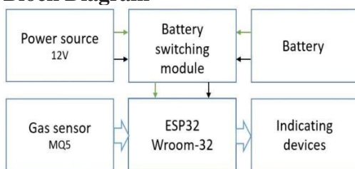
Block diagram of LPG gas leakage detection system
