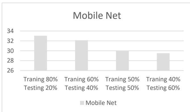
Fig 7: Impact of Data Size on Mobile Net
