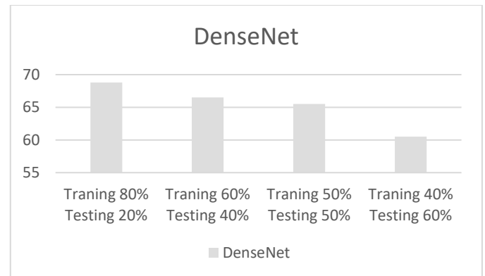
Fig 9: Impact of Data Size on DenseNet
