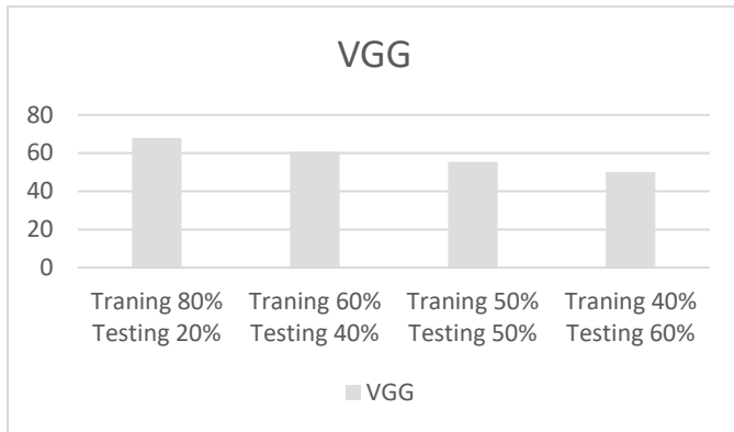
Fig 6: Impact of Data Size on VGG Net
