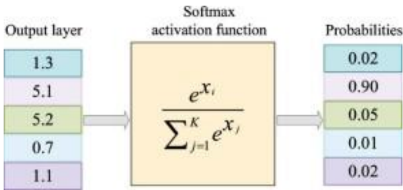
Fig 3. Softmax activation
