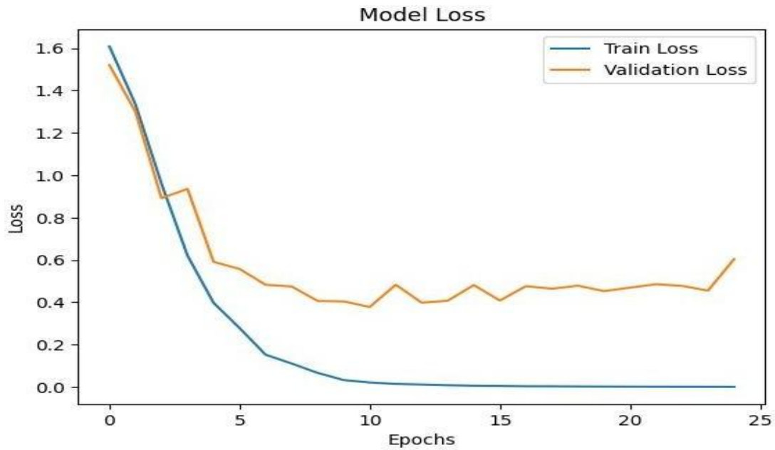
Fig 12. Model Loss
