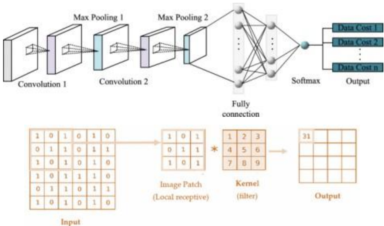
Fig 1. Convolution Layer
