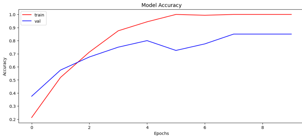
Fig 11. Model Accuracy
