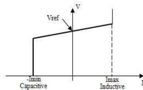
Fig. 1.6 - VI Characteristics
