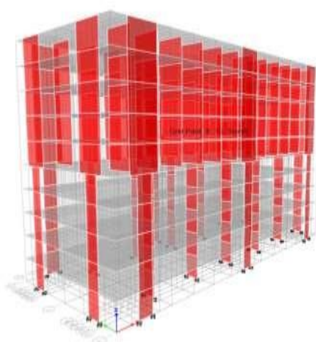
Transfer slab at 5 th floor
