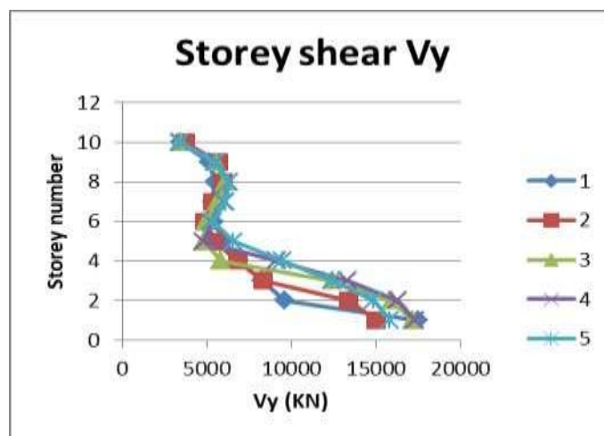
Fig 7. Storey shear distribution in y direction
