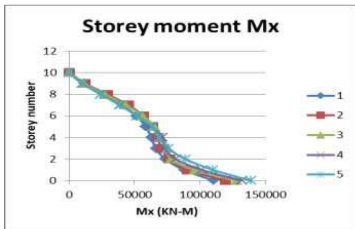
Fig 8. Storey moment distribution in x direction
