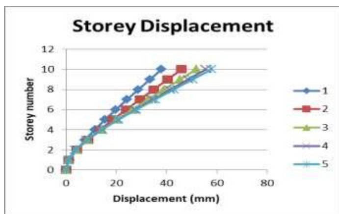
Fig 10. Storey displacement
