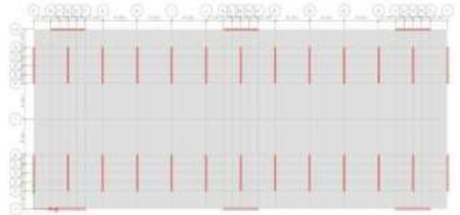
Fig 4. Position of shear wall above Transfer floor
