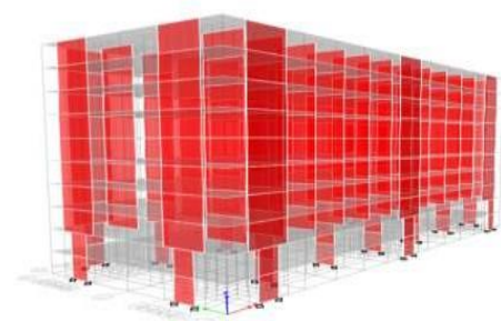
Transfer slab at 1 st floor
