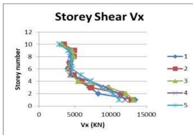
Fig 6. Storey shear distribution in x direction
