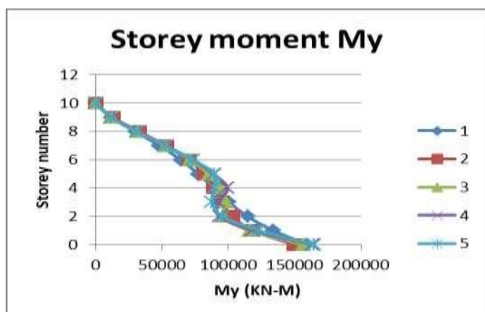
Fig 9. Storey moment distribution in y direction
