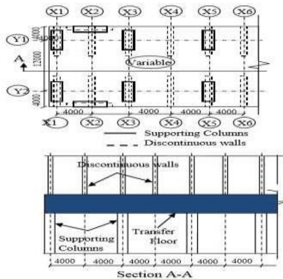
Fig 2. Transfer floor plan and cross section (transfer slab system)
