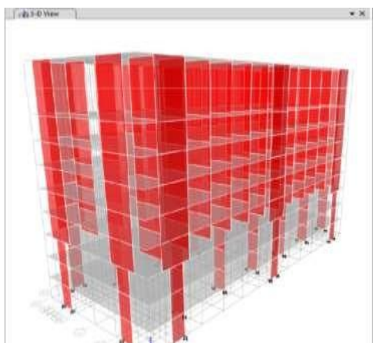
Transfer slab at 3 rd floor
