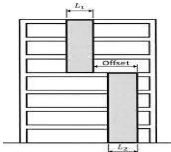
Fig. 1.9 In plane Discontinuity Irregularity
