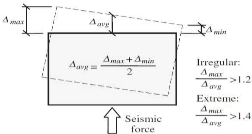
Fig. 1.1 Torsional irregularity
