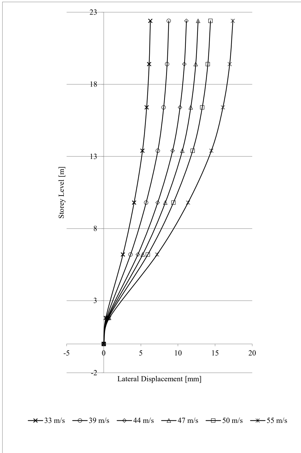
Fig. 4.4 Wind Response (Lateral Displacement) of Hybrid Irregular Frame – HIF at all Wind Zones in India
