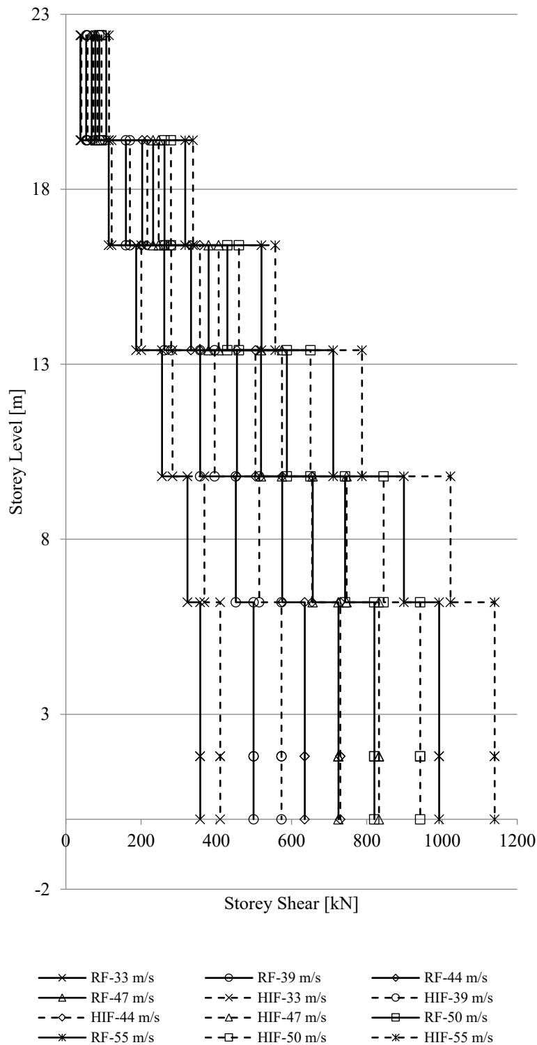
Fig. 4.9 Storey Shear Response of Regular (RF) and Hybrid Irregular (HIF) Frames under Wind Loads
