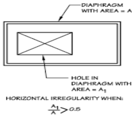
Fig. 1.3 Diaphragm Discontinuity
