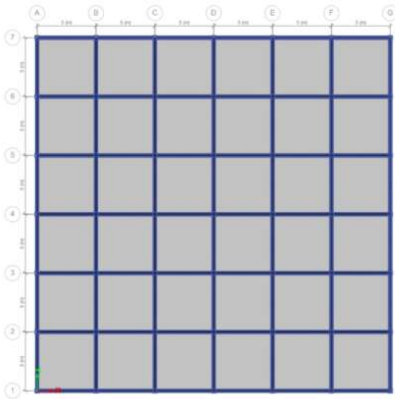
Fig. 3.3 (a) Plan of HIF
