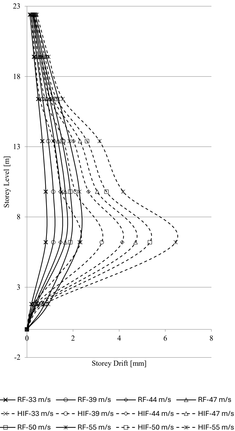
Fig. 4.8 Storey Drift Response of Regular (RF) and Hybrid Irregular (HIF) Frames under Wind Loads
