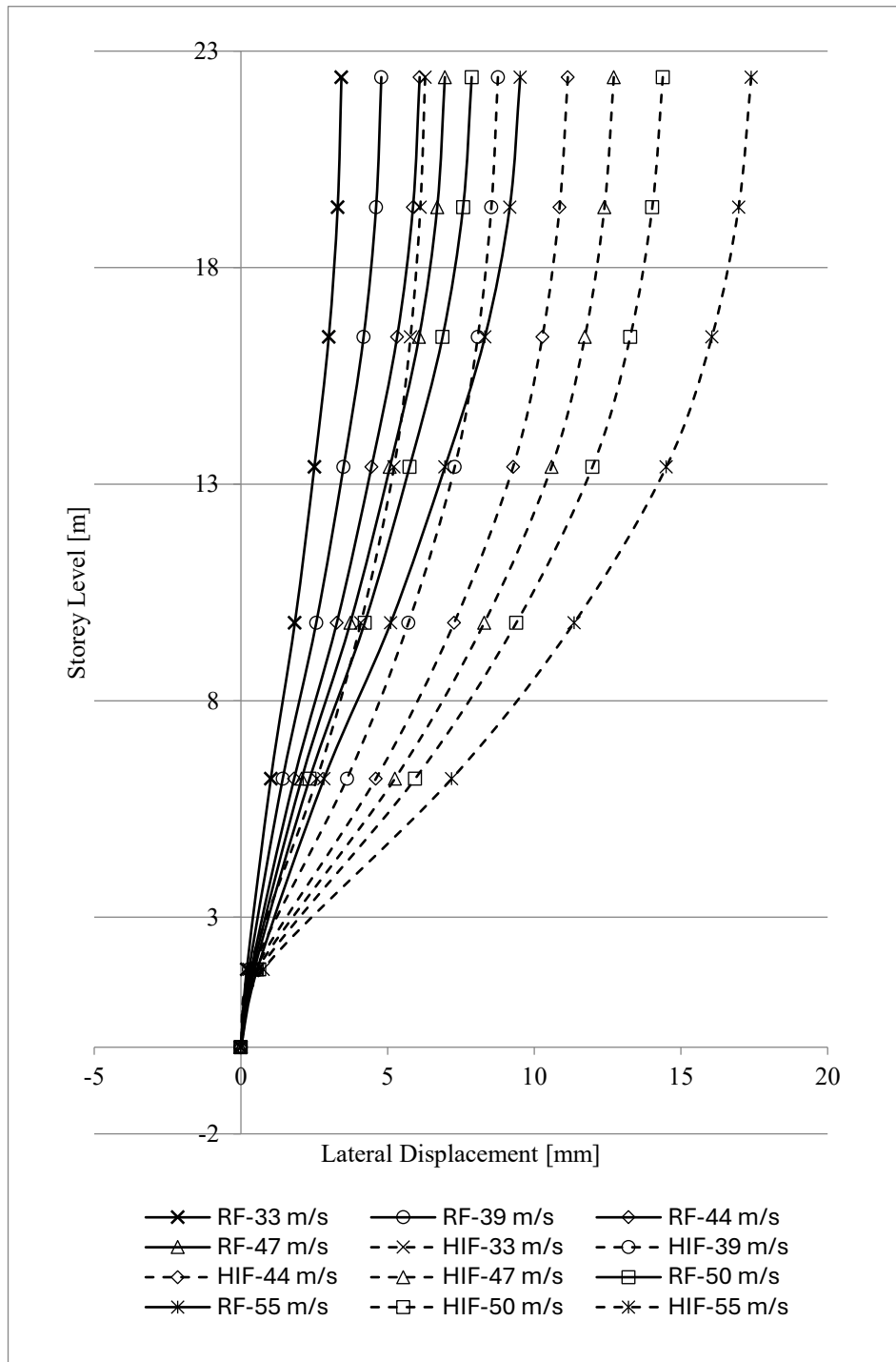
Fig. 4.7 Lateral Displacement Response of Regular (RF) and Hybrid Irregular (HIF) Frames under Wind Loads
