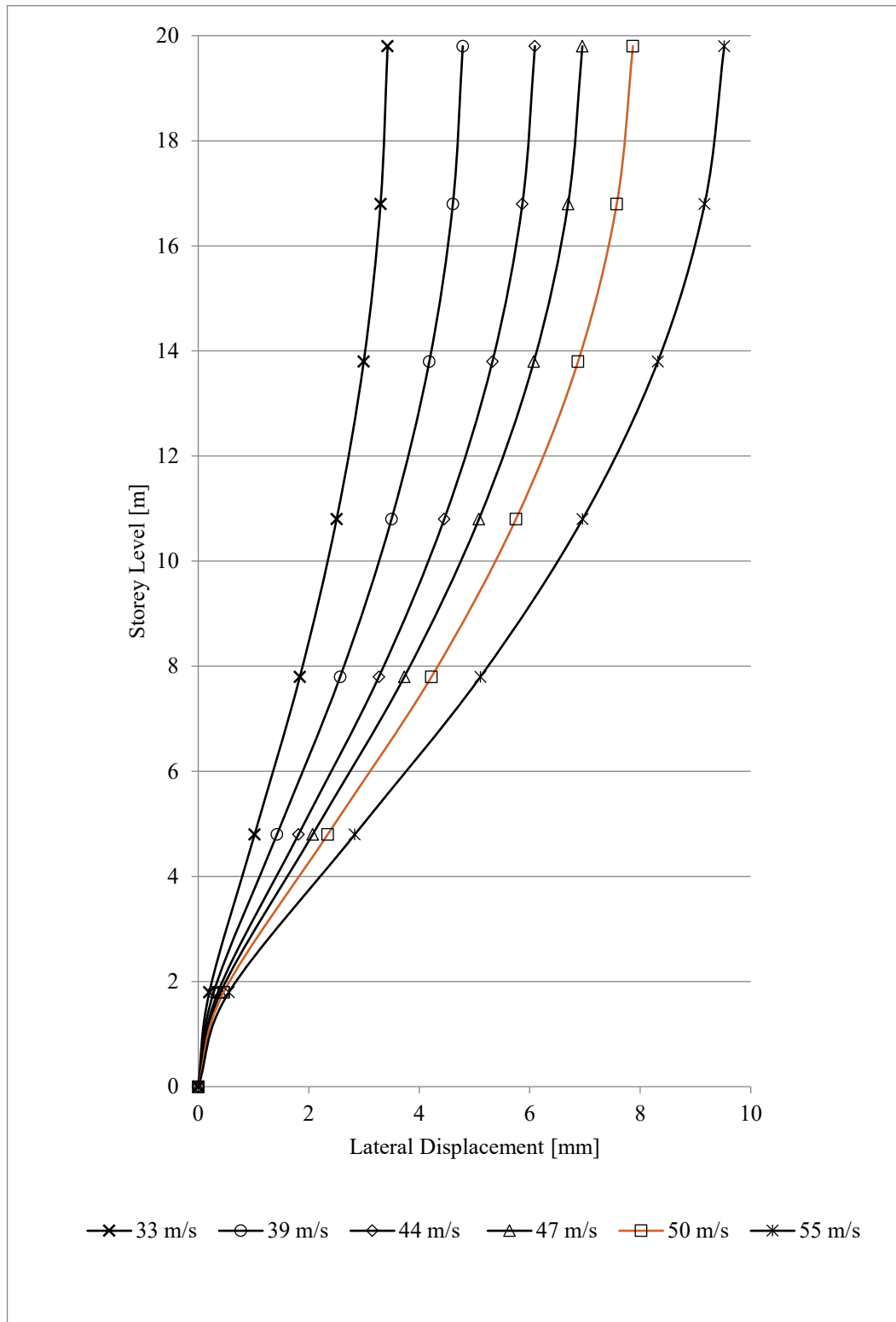
Fig. 4.1 Wind Response (Lateral Displacement) of Regular Frame – RF at all Wind Zones in India
