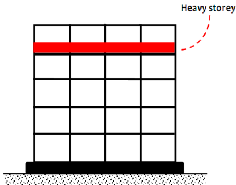
Fig. 1.7 Mass Irregularity
