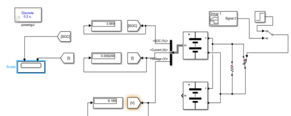
Figure 11.3:- CIRCUIT DIAGRAM OF DISCHARGE OF PARALLEL CONNECTED LEAD ACID-LITHIUM ION BATTERY WITH LOAD AS STEP SIGNAL FOR 140 HOURS
