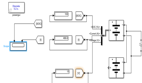
Figure 7.1:-CIRCUIT DIAGRAM OF LITHIUM ION BATTERY & LITHIUM ION BATTERY PARALLEL CHARGING FOR 1 HOUR
