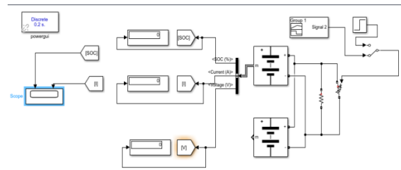
Figure 12.5:- CIRCUIT DIAGRAM OF DISCHARGE OF PARALLEL CONNECTED LITHIUM ION-LITHIUM ION BATTERY WITH LOAD AS STEP SIGNAL WITH RAMP START FOR 80 HOURS
