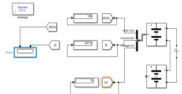
Figure 5.3:-CIRCUIT DIAGRAM OF LITHIUM ION BATTERY CONNECTED IN SERIES WITH LITHIUM ION BATTERY FOR 1 HOUR
