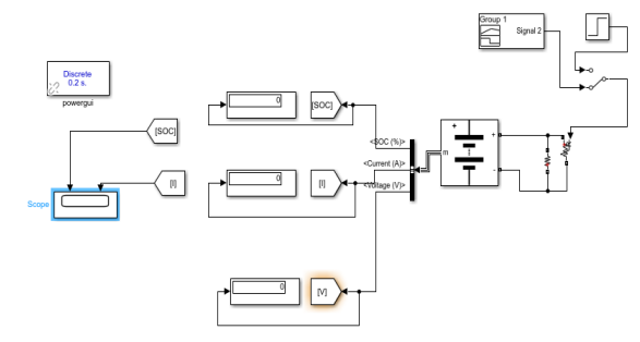
Figure 8.7:- CIRCUIT DIAGRAM OF DISCHARGE OF LITHIUM ION BATTERY WITH LOAD AS STEP SIGNAL WITH RAMP START FOR 20 HOURS
