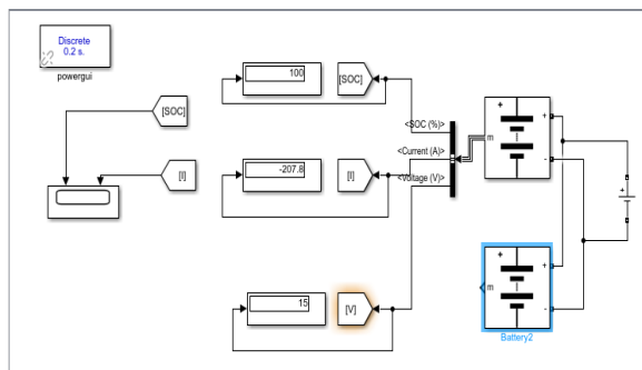
Figure 6.3:-CIRCUIT DIAGRAM OF LITHIUM ION BATTERY & LEAD ACID BATTERY PARALLEL CHARGING FOR 1 HOUR
