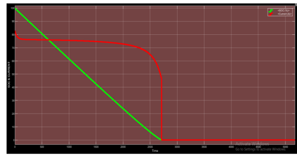
Figure 8.5:- SOC & CURRENT WAVEFORM OF LITHIUM ION BATTERY CONNECTED TO STEP SIGNAL FOR 25 HOURS
