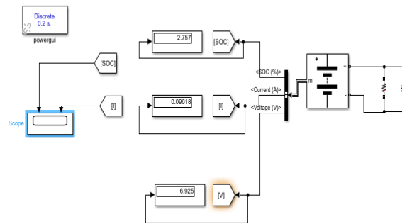
Figure 8.1:- CIRCUIT DIAGRAM OF DISCHARGE OF LITHIUM ION BATTERY WITH LOAD RESISTANCE 72 OHMS FOR 500 HOURS
