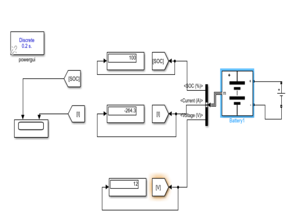
Figure 3.2.3 :- CIRCUIT DIAGRAM OF LITHIUM ION BATTERY CHARGING FOR 425 SECONDS
