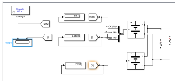
Figure 12.1:- CIRCUIT DIAGRAM OF DISCHARGE OF PARALLEL CONNECTED LITHIUM ION-LITHIUM ION BATTERY WITH LOAD AS 72 OHMS FOR 500 HOURS
