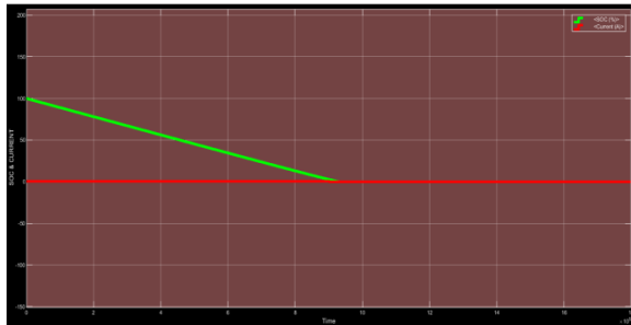
Figure 10.3:- SOC & CURRENT WAVEFORM OF DISCHARGE OF LITHIUM ION-LITHIUM ION ACID SERIES BATTERY WITH LOAD AS STEP SIGNAL FOR 500 HOURS
