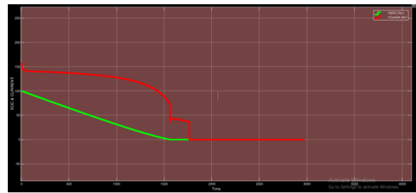
Figure 9.4:- SOC & CURRENT WAVEFORM OF DISCHARGE OF LEAD ACID-LITHIUM ION ACID SERIES BATTERY WITH LOAD AS STEP SIGNAL WITH RAMP START FOR 500 HOURS
