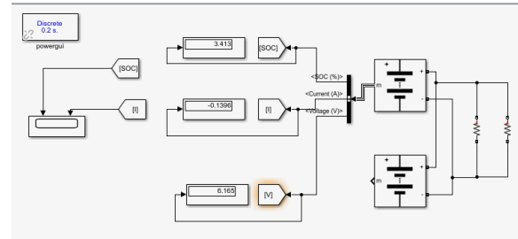
Figure 11.1:- CIRCUIT DIAGRAM OF DISCHARGE OF PARALLEL CONNECTED LEAD ACID-LITHIUM ION BATTERY WITH LOAD RESISTANCE 72 OHMS FOR 470 HOURS
