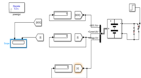
Figure 8.3:- CIRCUIT DIAGRAM OF DISCHARGE OF LITHIUM ION BATTERY WITH LOAD AS STEP SIGNAL FOR 25 HOURS
