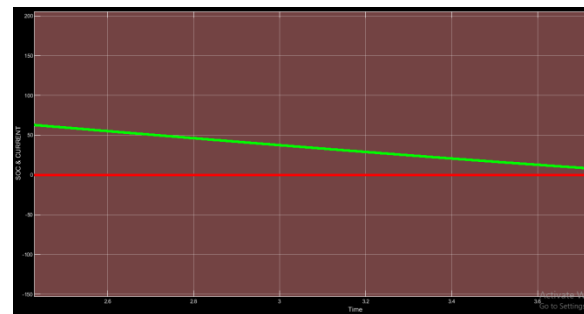
Figure 11.2:- SOC & CURRENT WAVEFORM OF DISCHARGE OF PARALLEL CONNECTED LEAD ACID-LITHIUM ION BATTERY WITH LOAD RESISTANCE 72 OHMS FOR 470 HOURS
