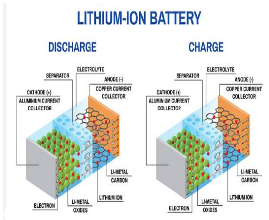
Figure1.1:-CHARGING AND DISCHARGING OF LITHIUM ION BATTERY
