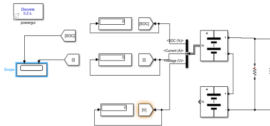
Figure 9.1:- CIRCUIT DIAGRAM OF DISCHARGE OF LEAD ACID-LITHIUM ION ACID SERIES BATTERY WITH LOAD RESISTANCE OF 72 OHMS FOR 500 HOURS
