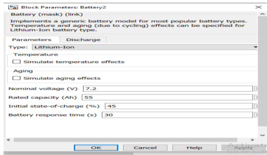
Figure 6.1:-DETAIL SPECIFICATION OF LITHIUM ION BATTERY
