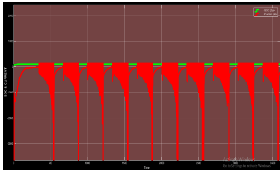
Figure 4.4:-SOC & CURRENT WAVEFORM OF LEAD ACID BATTERY CONNECTED SERIES WITH LITHIUM ION BATTERY FOR 1 HOUR
