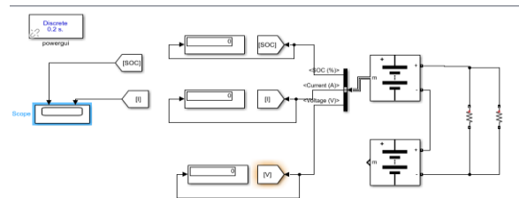
Figure10.1:- CIRCUIT DIAGRAM OF DISCHARGE OF LITHIUM ION-LITHIUM ION ACID SERIES BATTERY WITH LOAD RESISTANCE OF 72 OHMS FOR 500 HOURS
