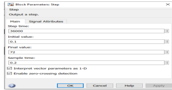
Figure 8.4:- IMAGE SHOWING DETAILS OF STEP SIGNAL
