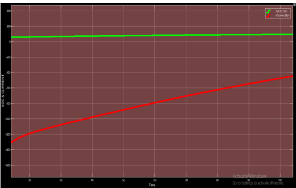
Figure 3.2.4:- SOC & CURRENT WAVEFORM OF LITHIUM ION BATTERY CHARGING FOR 135 SECONDS IS CAPTURED AND DISPLAYED FOR BETTER OBSERVATION
