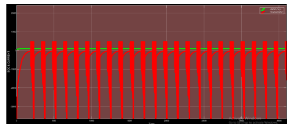
Figure 5.4:-SOC & CURRENT WAVEFORM OF LITHIUM ION BATTERY CONNECTED IN SERIES WITH LITHIUM ION BATTERY FOR 1 HOUR
