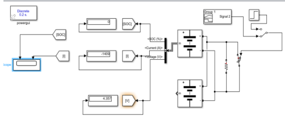
Figure 11.5:- CIRCUIT DIAGRAM OF DISCHARGE OF PARALLEL CONNECTED LEAD ACID-LITHIUM ION BATTERY WITH LOAD AS STEP SIGNAL WITH RAMP START FOR 200 HOURS
