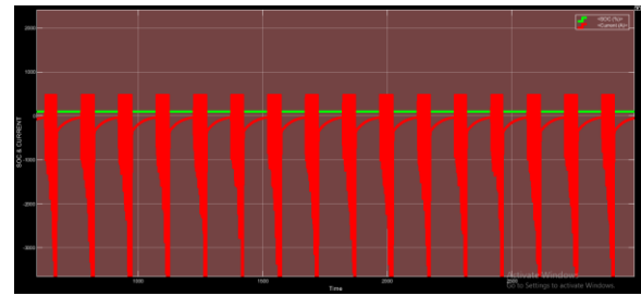
Figure 7.2:-SOC & CURRENT WAVEFORM OF LITHIUM ION BATTERY & LITHIUM ION BATTERY FOR PARALLEL CHARGING FOR 1 HOUR
