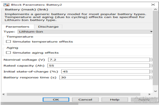
Figure 3.2:- DETAIL SPECIFICATION OF LITHIUM ION BATTERY
