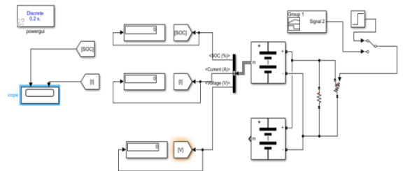
Figure 12.3:- CIRCUIT DIAGRAM OF DISCHARGE OF PARALLEL CONNECTED LITHIUM ION-LITHIUM ION BATTERY WITH LOAD AS STEP SIGNAL FOR 6 HOURS
