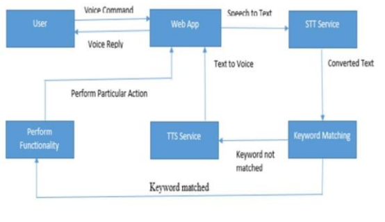
Architecture of the Web Application
