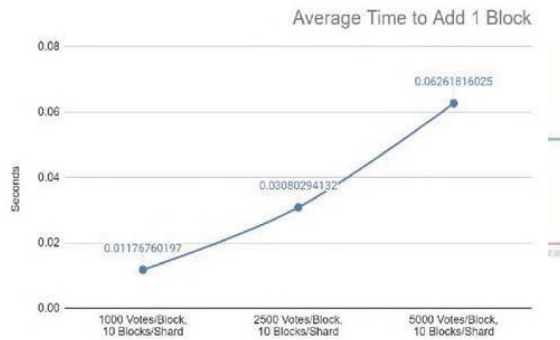
Fig. 4. Average time taken to add one (1) block when handling different quantities of votes stored per block.
