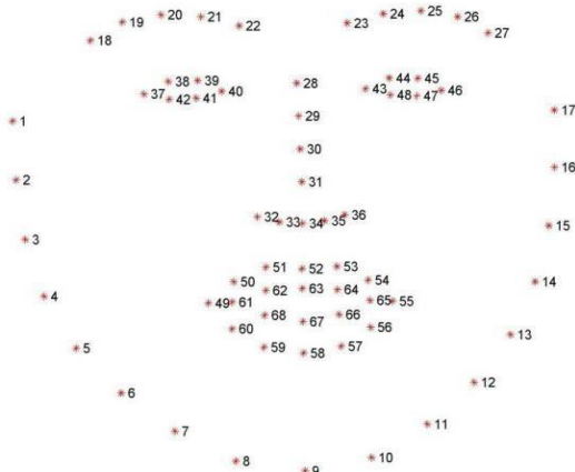
Fig.2. Facial Landmark
