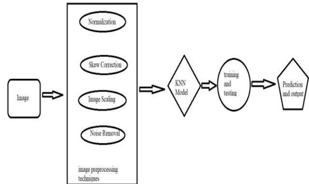
Fig.3.Methodology
