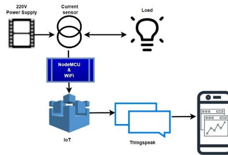
Figure 1: Block Diagram
