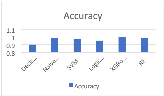
Fig2: Accuracy comparison of different models.
