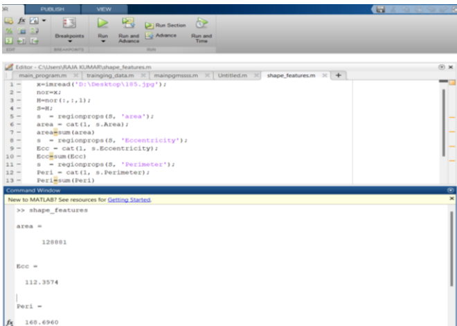
Fig 9: Shape Features
