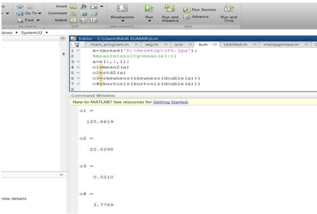
Fig 8: Colour Features
