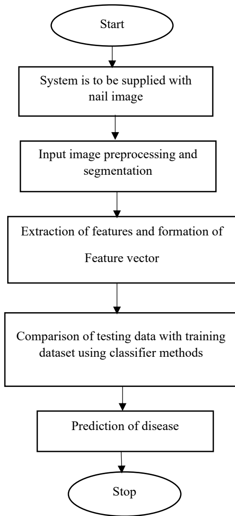
Fig 1: Flowchart
