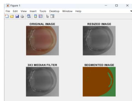
Fig 7: Mixed Plot
