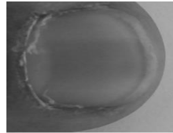
Fig 5: Preprocessed image
