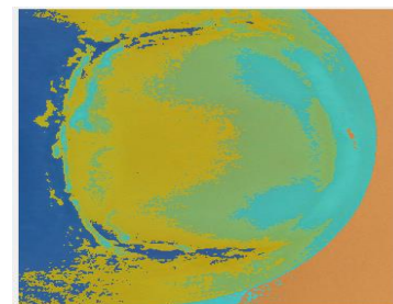
Fig 6: Segmented image
