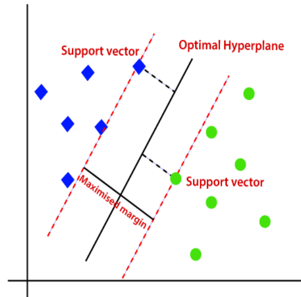
Fig 2: Multiclass SVM
