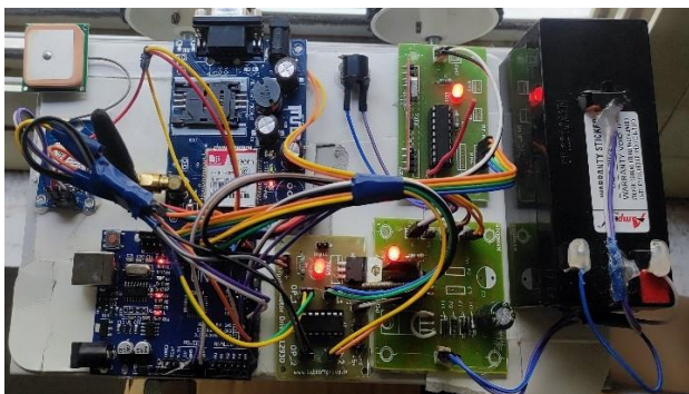
Fig.7.hardware kit
