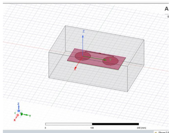
Figure .4. Two element Planner array HFSS model
