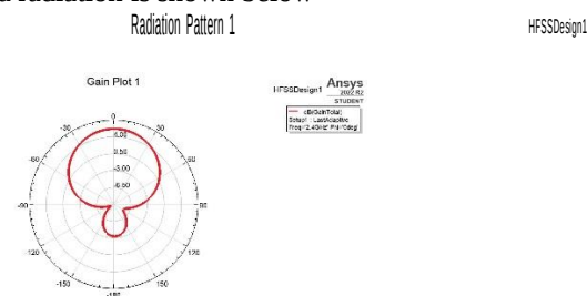
Figure.8. Radiation pattern
