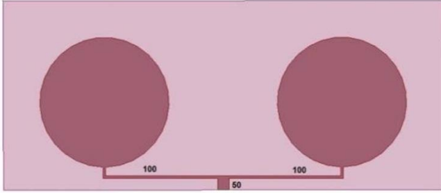
Figure.1. Two elements corporate feed microstrip antenna array
