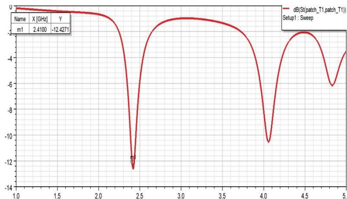
Figure.6. Return loss
