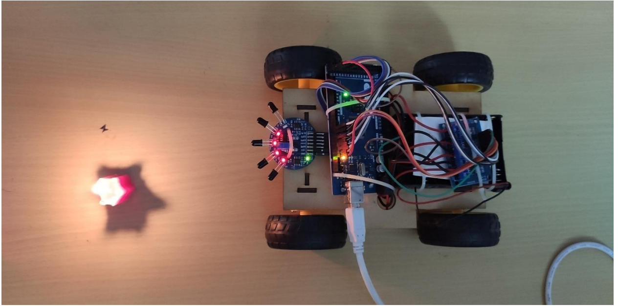
Fig 5: Robot moves near to object
