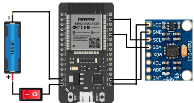
Fig. 1. Transmitter circuit.
