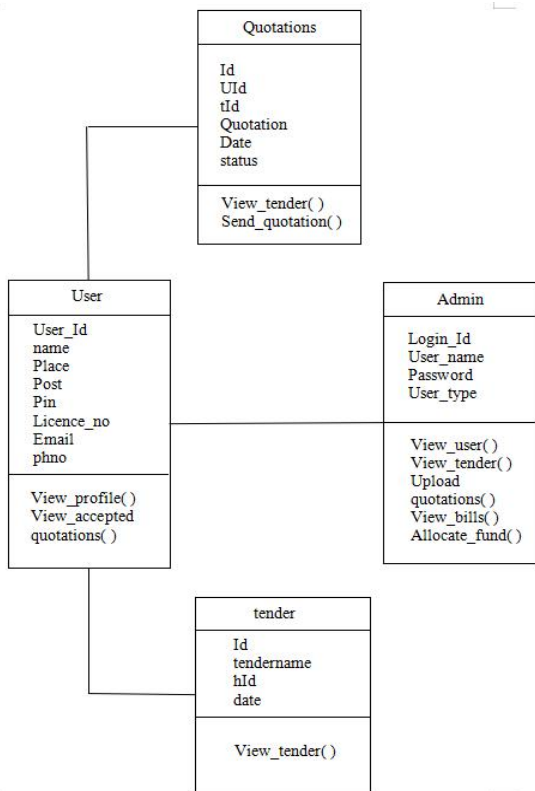
Figure 6. Class diagram of the system
