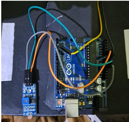
LDR Interface to Arduino
