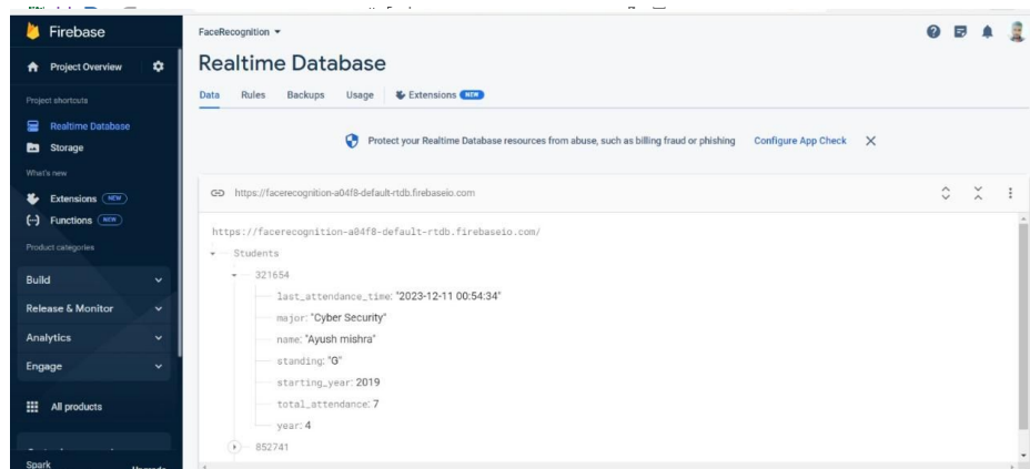
Fig.4. Face Recognition
