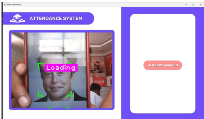
Fig.3. Face Detection
