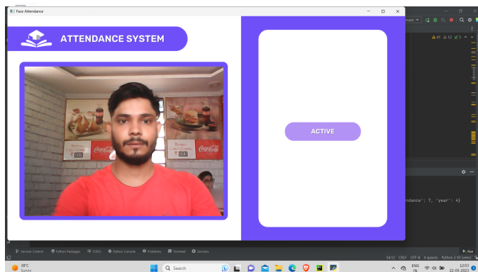
Fig.4. Face Recognition
