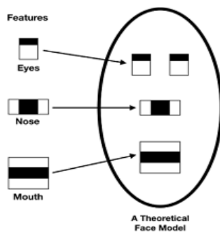
Fig.2. Haar Features
