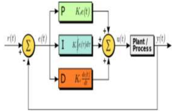
FIGURE 5: PID CONTROLLER
