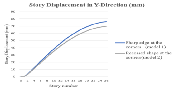
Fig.4.8: Story Displacement in Y-Direction
