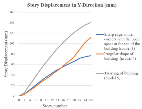
Fig.4.14: Story Displacement in Y-Direction
