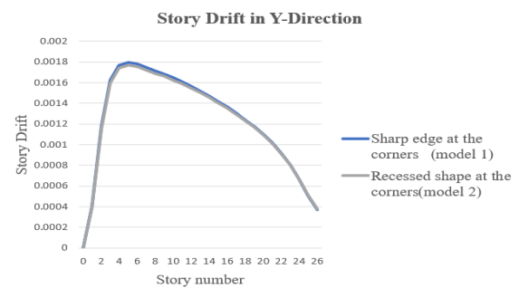
Fig.4.4: Story Drift in Y-Direction
