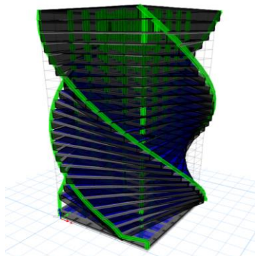
Fig.3.3: sharp edge at the corners with the open space of the building(model 3) and Fig.3.4: irregular shape of the building (model4)
