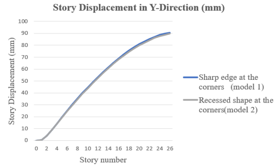
Fig.4.2: Story Displacement in Y-Direction
