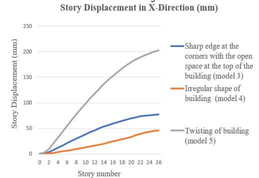
Fig.4.19: Story Displacement in X-Direction
