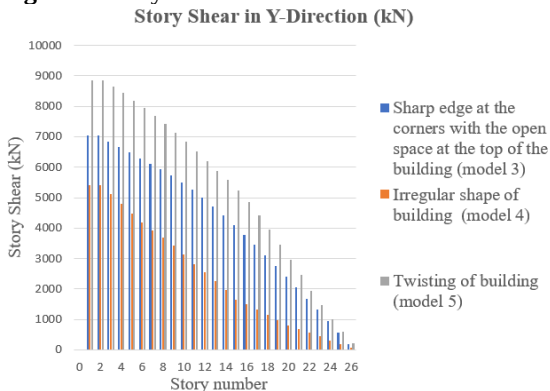
Fig.4.23: Story Shear in Y-Direction
