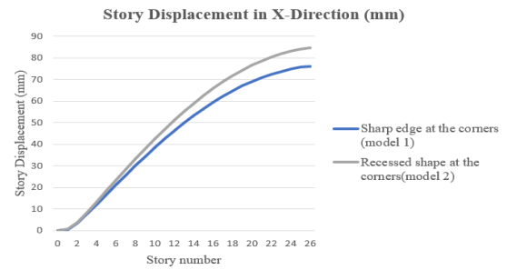
Fig.4.7: Story Displacement in X-Direction
