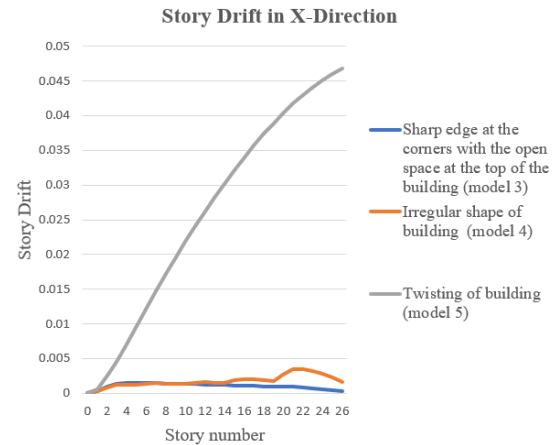
Fig.4.15: Story Drift in X-Direction
