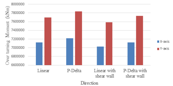
Fig 4.17: Over turning moment in both directions for cut shape at the corners of the building
