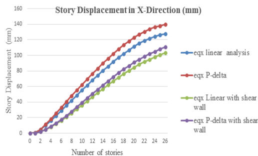
Fig 4.3: Displacement in X-direction at sharp edge
