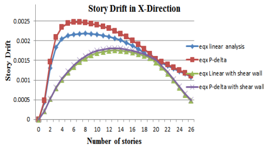
Fig 4.7: Story drift in X-direction at sharp edge
