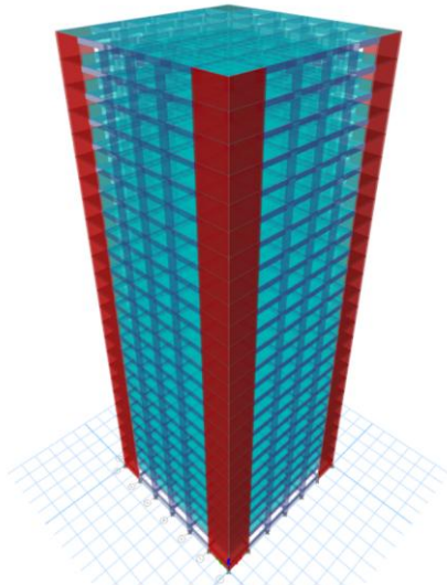
Fig 3.2: 3D view of model with shear wall (model1b)
