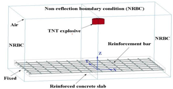
Fig. 2. Finite element model.
