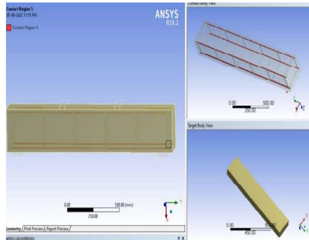
Figure 4: Contact between concrete and rebars
