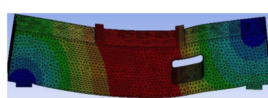
Figure 9: Deformation of beam with CFRP inside wrapping of beam
