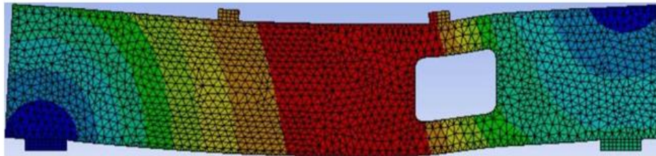
Figure 8: Deformation of beam with opening
