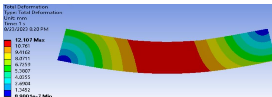
Figure 7: Deformation of beam without opening
