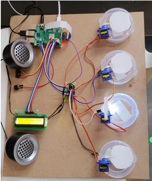
FIG 13: Hardware Unit
