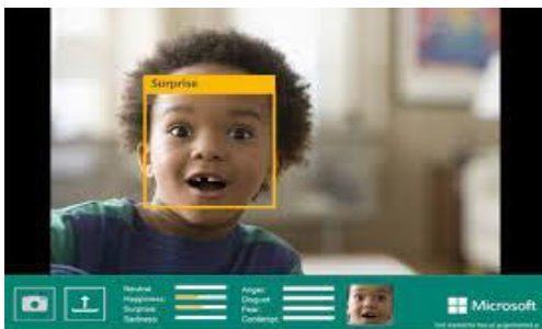
Figure 1.1: Emotion recognition
