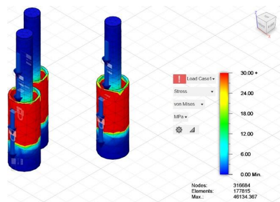
Figure(2) analysis of landing gear
