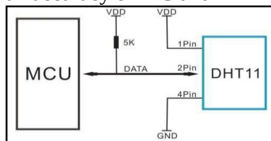
Fig 2. TEMPERATURE SENSOR
