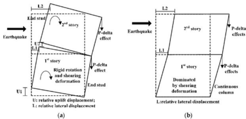
Fig.1.3: Deformation of CFS shear wall
