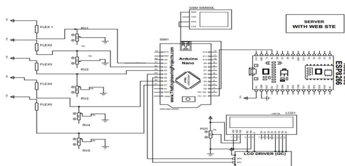
Fig. 5 Circuit Diagram
