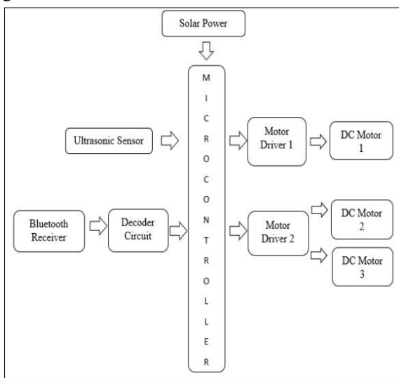
Figure 1: The proposed block diagram of river cleaning robot
