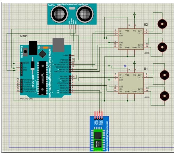
Figure 3: Proteus Circuit Simulation
