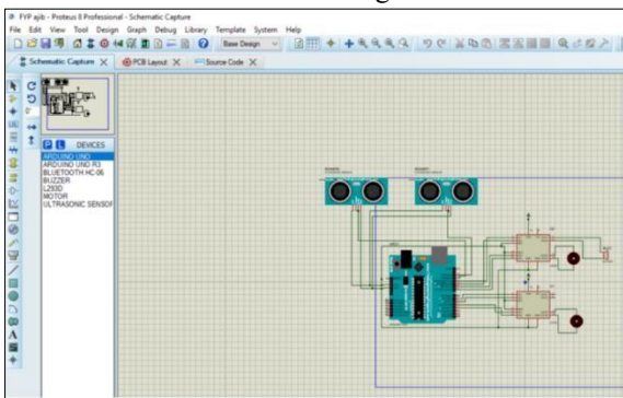
Figure 2: The proposed circuit diagram
