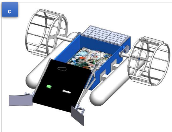
Figure 4: Final design (a)Top View, (b)Front View and (c)Isometric View
