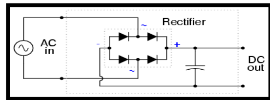
Figure 2: AC to DC converter
