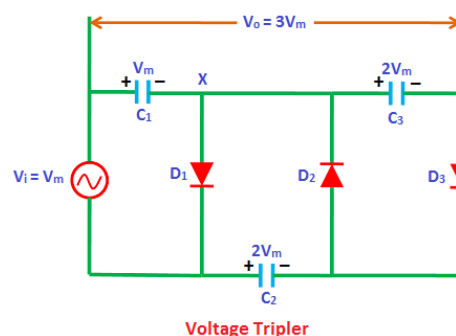
Fig Voltage multiplier Voltage multiplier
