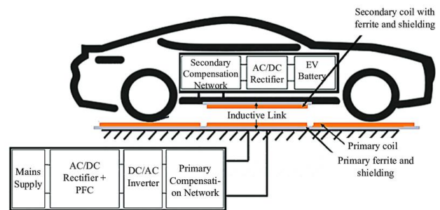
Fig 3 Construction of contactless EV charging system
