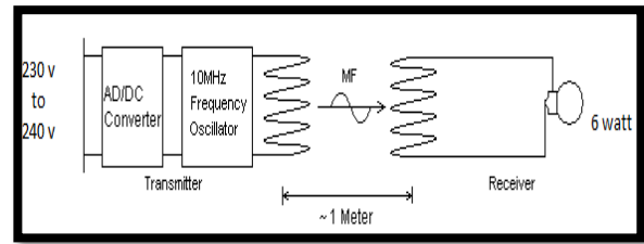
Figure 3: Wireless Energy Charger
