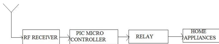
Fig -2. Block diagram for RF receiver section
