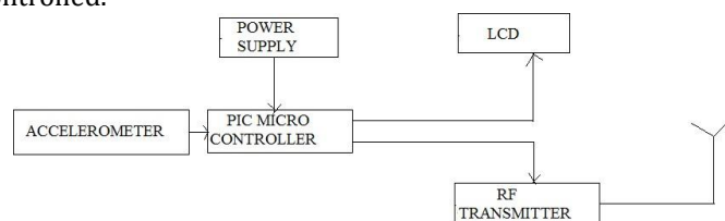
Fig -1. Block diagram for RF transmitter section
