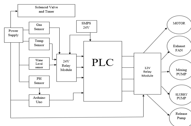
FIG. 01 BLOCK DIAGRAM
