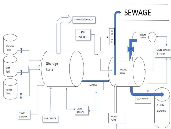
Figure 2 Flow Diagram of the system
