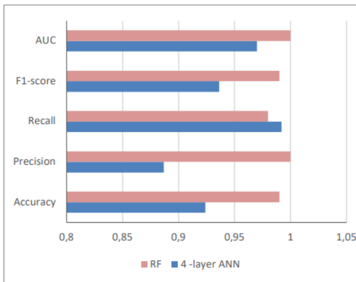
Fig. 8. A comparison chart of evaluation metrics of machine RF and 4-layer ANN algorithms
