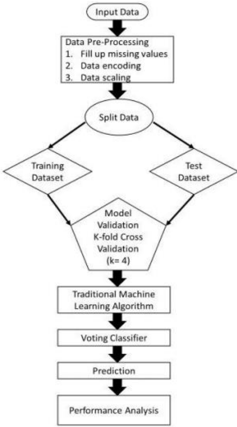
Fig. 3. Schematic working process diagram of our system
