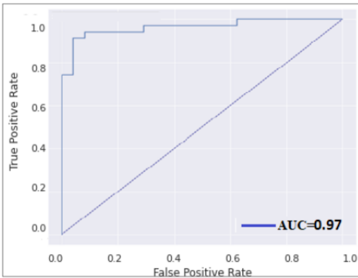
Fig. 7. The area under roc curve for 4-layer ANN method.
