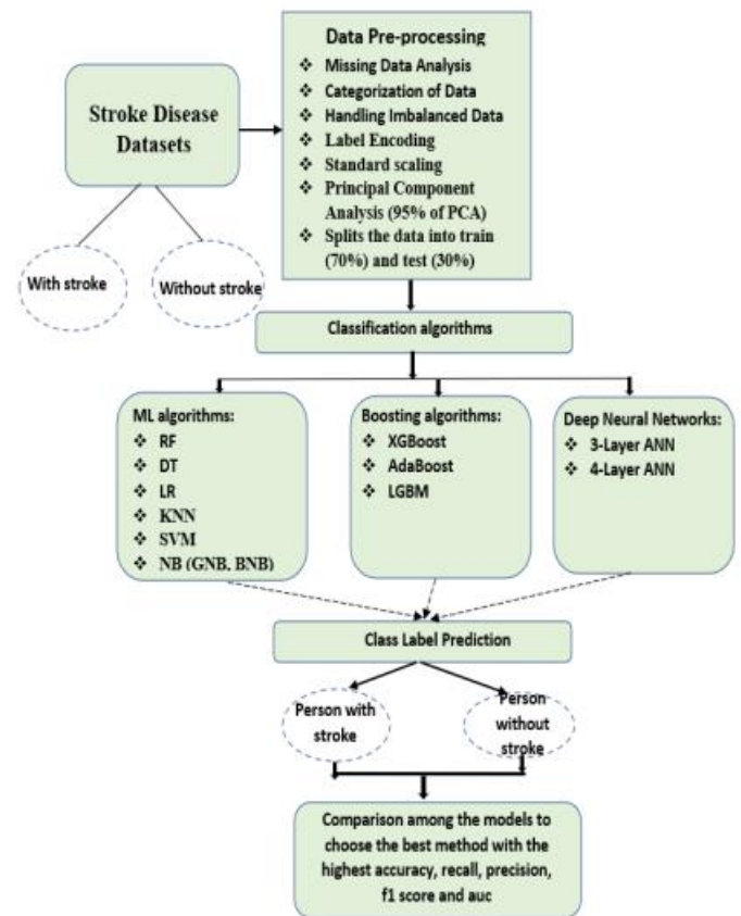
Fig. 2. The workflow of the proposed methodology.
