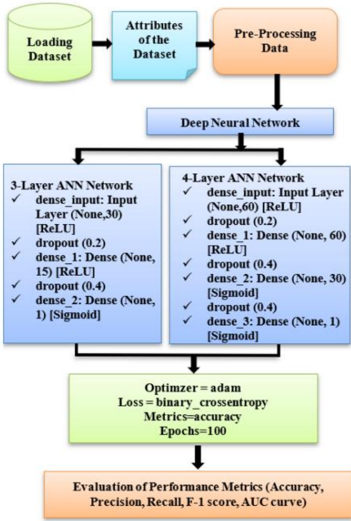
Fig. 4. The flowchart of the two proposed ANN techniques
