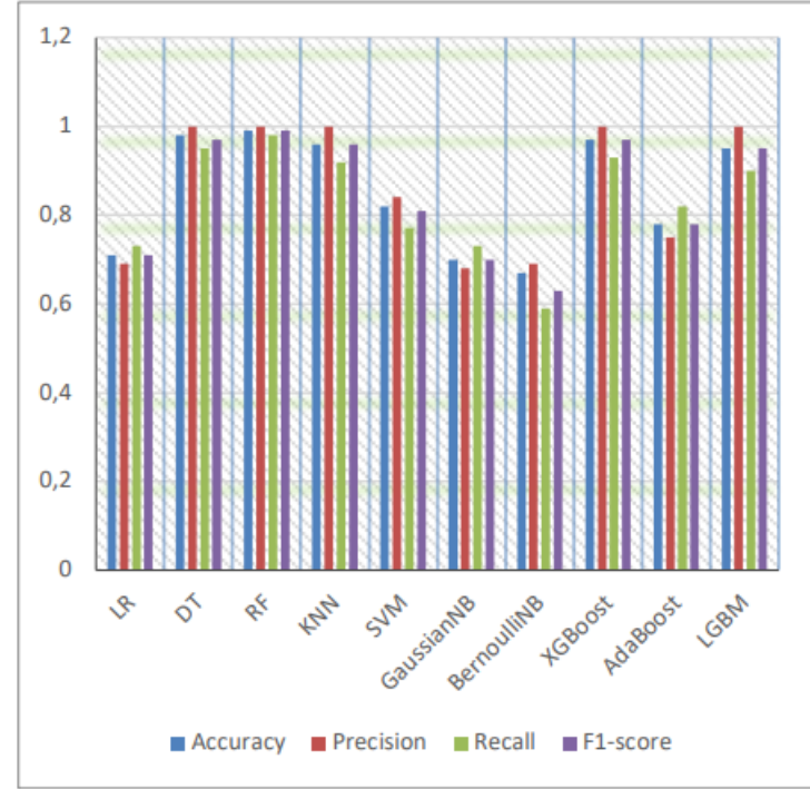
Fig. 5. A comparison chart of evaluation metrics of machine learning algorithms.
