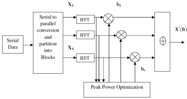
Fig. 3. PTS Block Diagram
